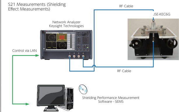
System Wiring Example for JSE-KEC6G (for Transmission Loss Measurements S21)
