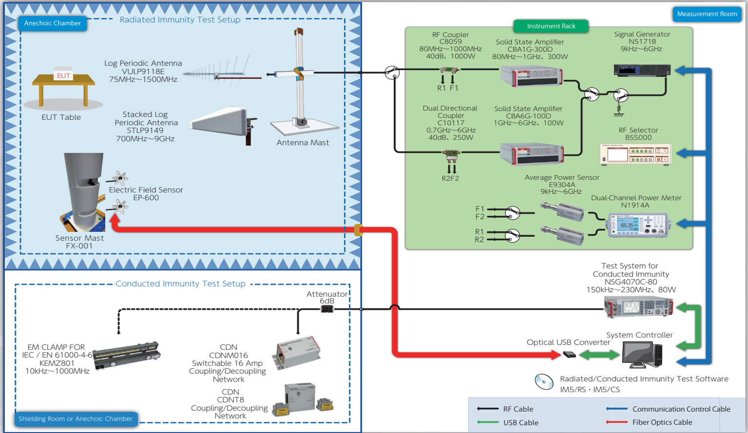
EMS Automatic Measurement System
