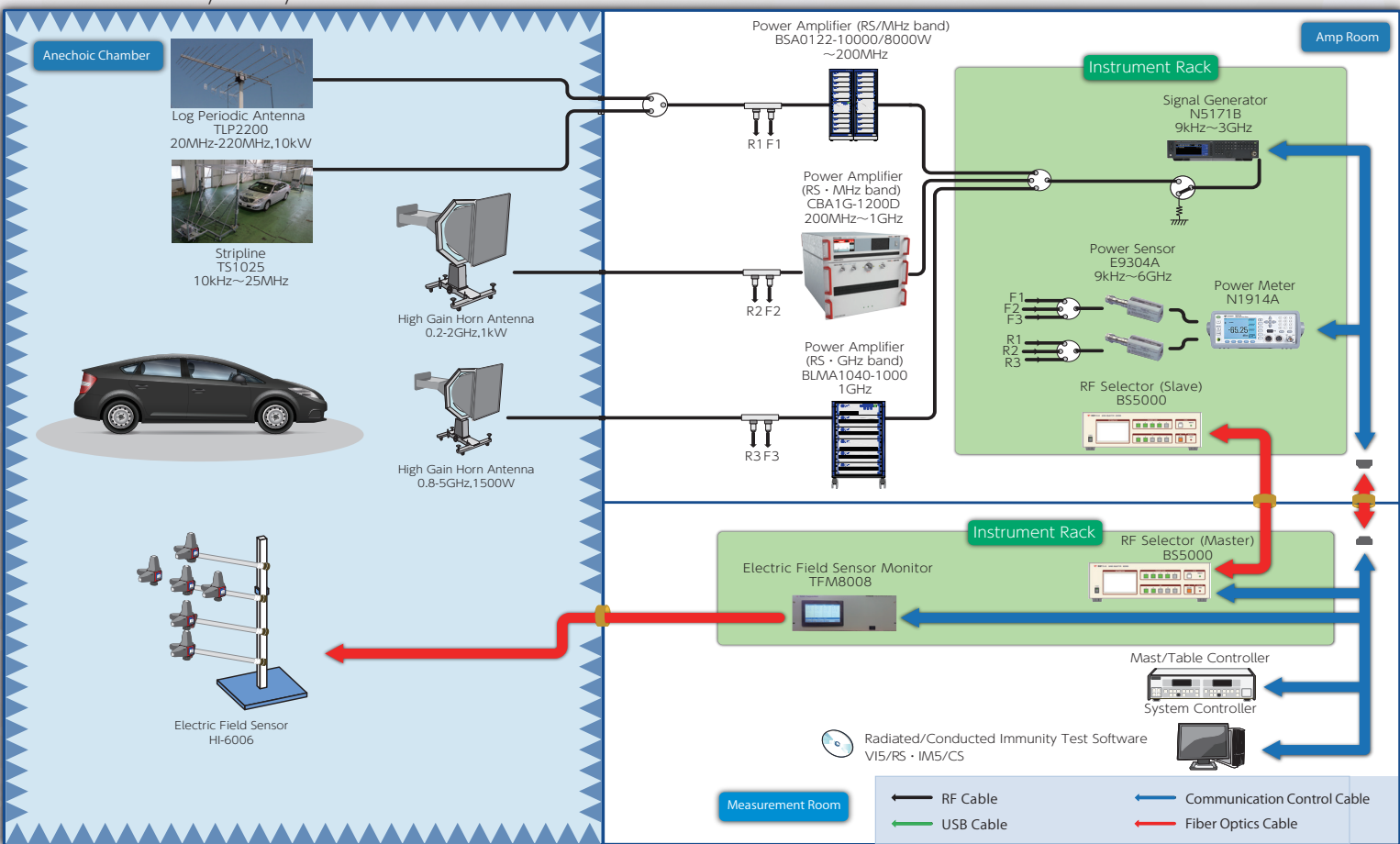
Full Vehicle Immunity Test System
