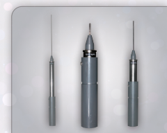
CV07-430 430MHz 1/4 λ Sleeve antenna CV07-1880 1880MHz 1/4 λ Sleeve antenna CV07-835 835MHz 1/4 λ Sleeve antenna
